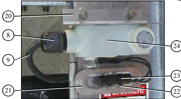
Rear discharge switch (open to show mercury switch).
